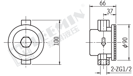
CWU-A25X60
