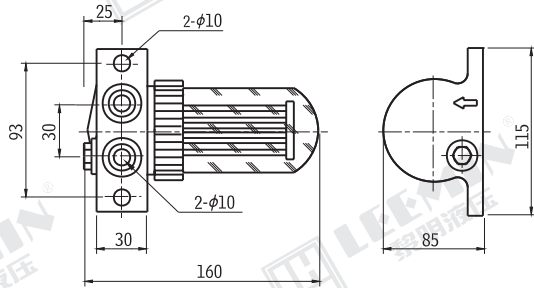
CWU-10X100B
